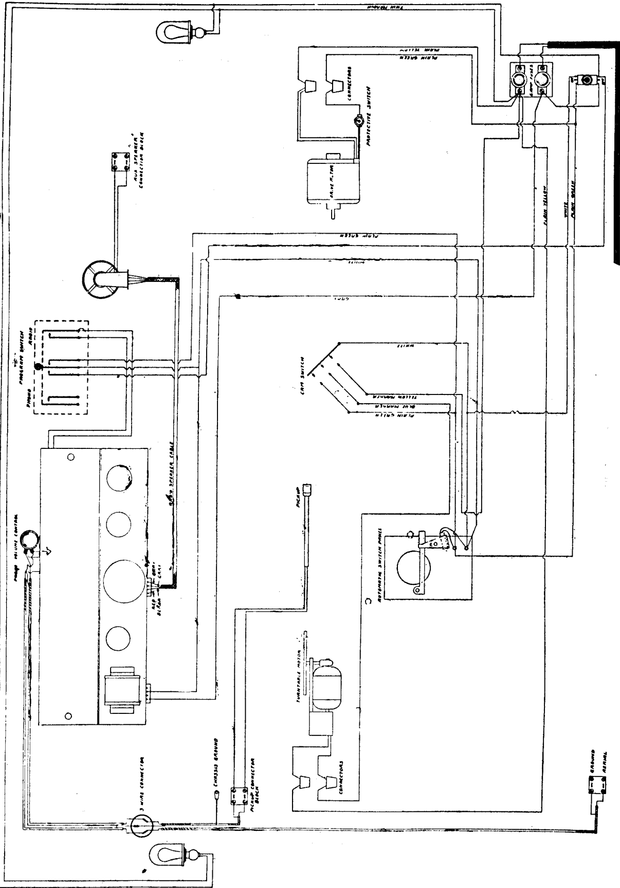
WIRING DIAGRAM *111 CAPEHART AMPERION
